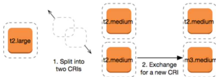
A t2 large RI, with a normalization factor of four, splits into two t2.medium RIs, each with a factor of two.
