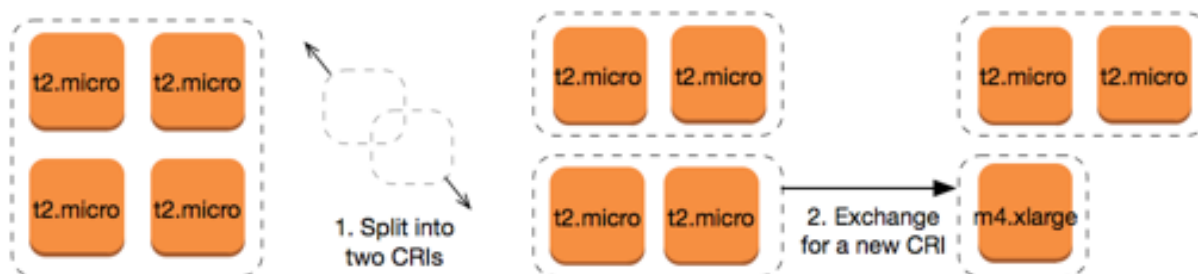
Splitting a four-instance t2.micro RI into a two-instance t2.micro RI and one m4.xlarge RI. (Source: AWS )
